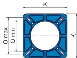
Burner flange
