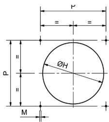
Recommended boiler hole
